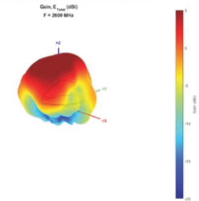
TYPICAL 3D PATTERN - LTE 1 2600 MHZ
